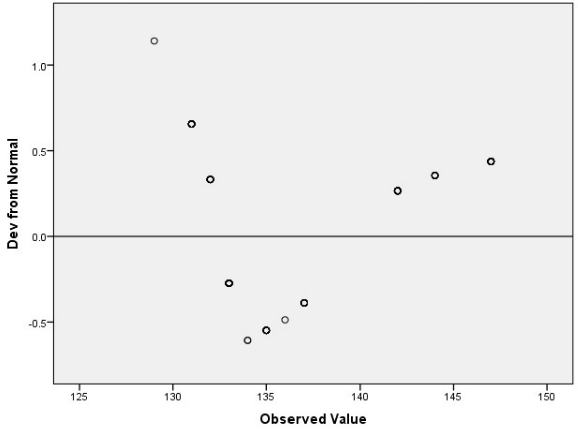
Detrended Normal Q-Q Plot of NORMALITAS
