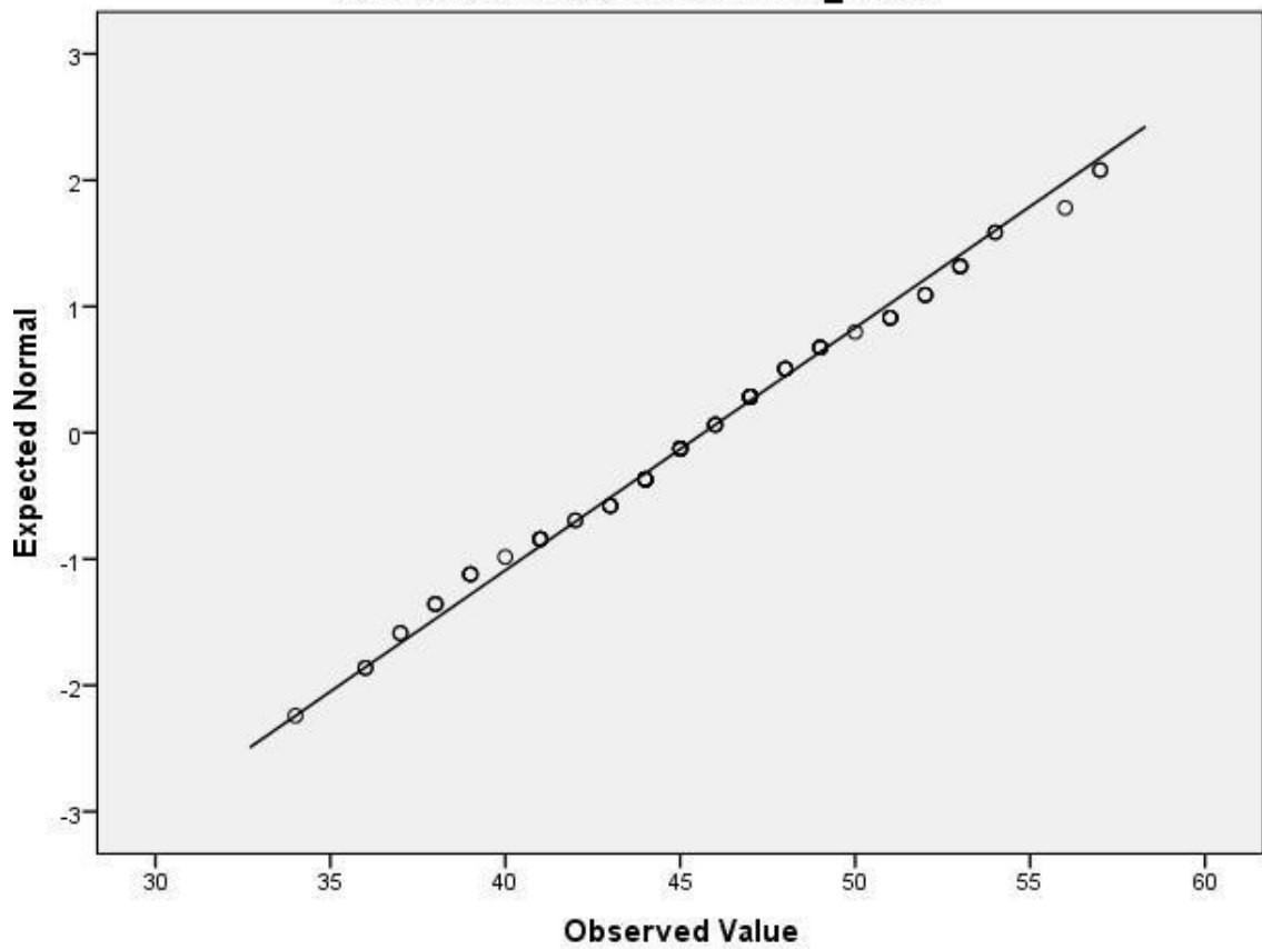
Normal Q-Q Plot of DUKUNGAN_FULL
