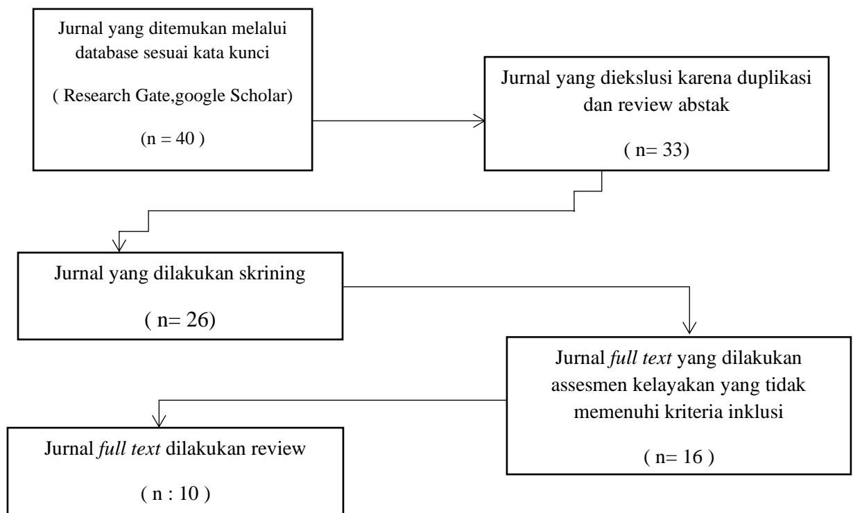
Gambar 3.1 Flow Gram
