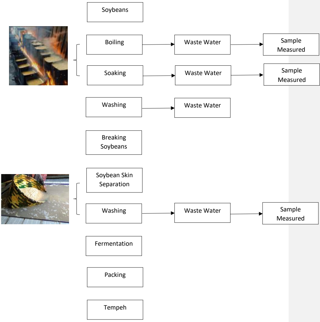
Figure 1 Tempeh Production Processes and Samples Measured
