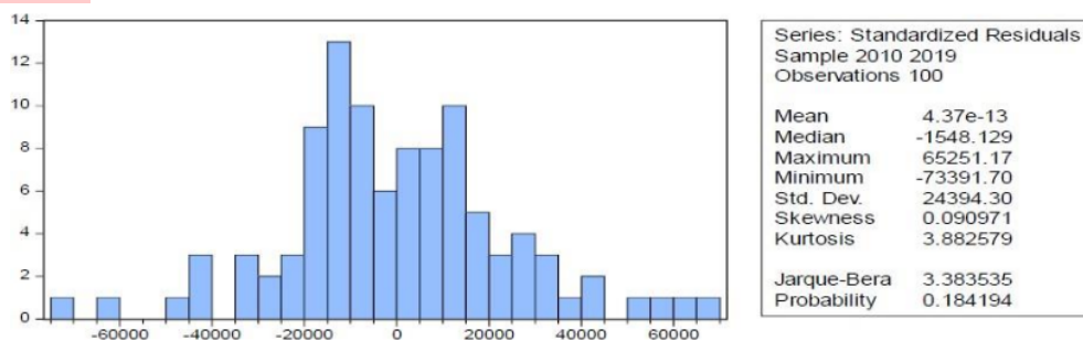
Figure 2. Histogram of Normality Test
