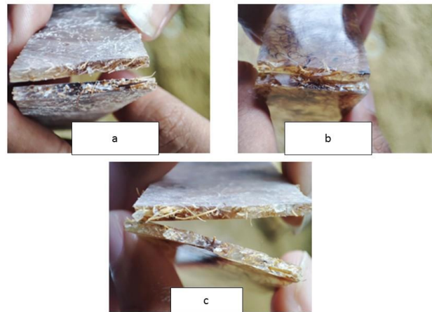
FIGURE 6. fracture of specimen during tensile testing a) 2 hours immersion time . b) 4 hours immersion time, c) 6 hours immersion time
