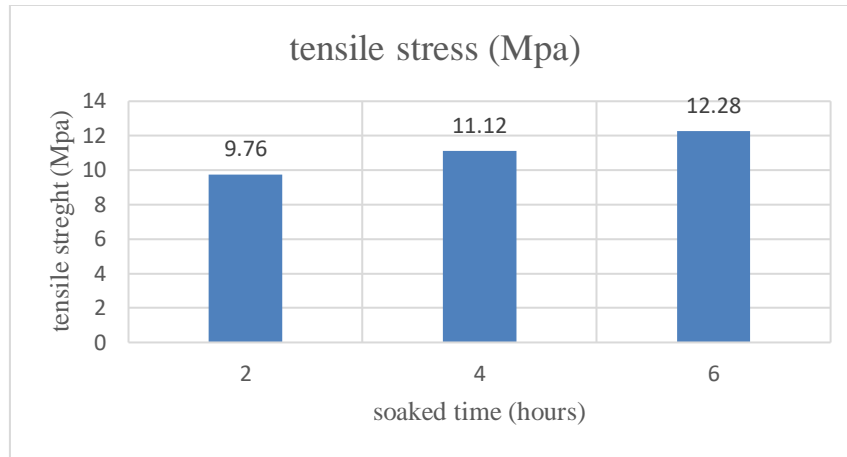
FIGURE 5. Tensile strenght of composite reinforcement OPEFB fiber
