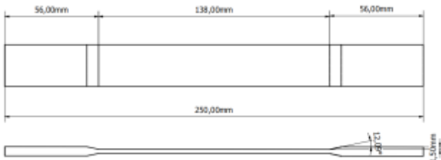
Gambar 4. Dimensi Spesimen Uji Tarik (ASTM D3039)
