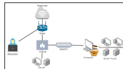
Figure 2. Honeypot network topology design
