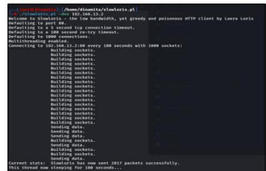
Figure 9. TCP attack testing
