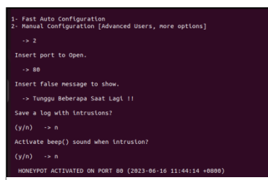
Figure 7. Configure HoneyPot Ports
