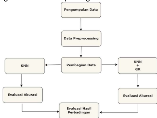
Gambar 1 Alur Penelitian
