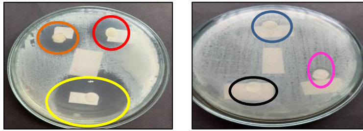
Figure 2. Observation result of inhibition of gelinggang extract on S. aureus bacteria
