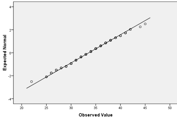
Normal Q-Q Plot of Kemandirian
