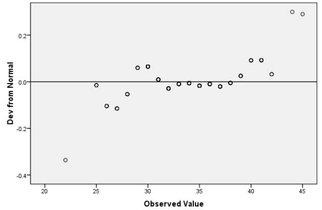
Detrended Normal Q-Q Plot of Kemandirian
