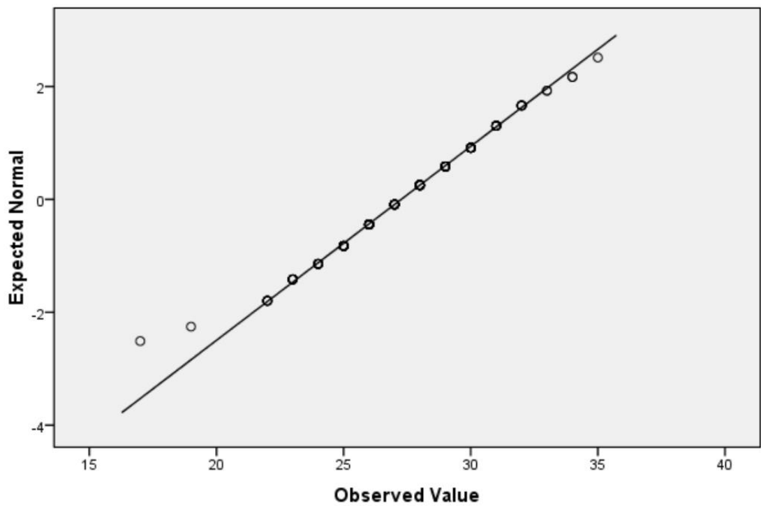
Normal Q-Q Plot of Perilaku Agresif
