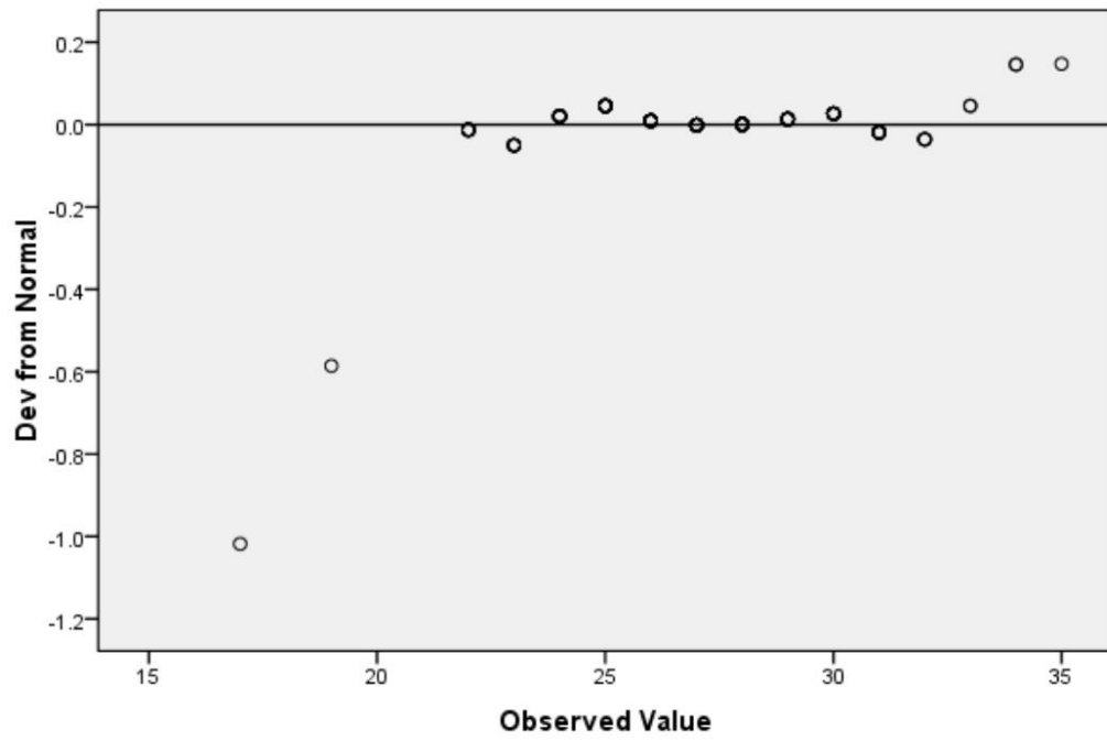
Detrended Normal Q-Q Plot of Perilaku Agresif
