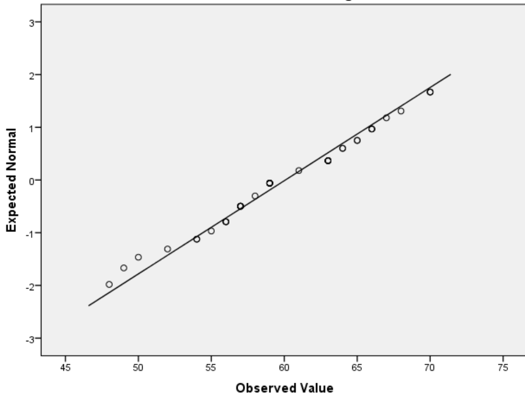
Normal Q-Q Plot of Peran Orang Tua
