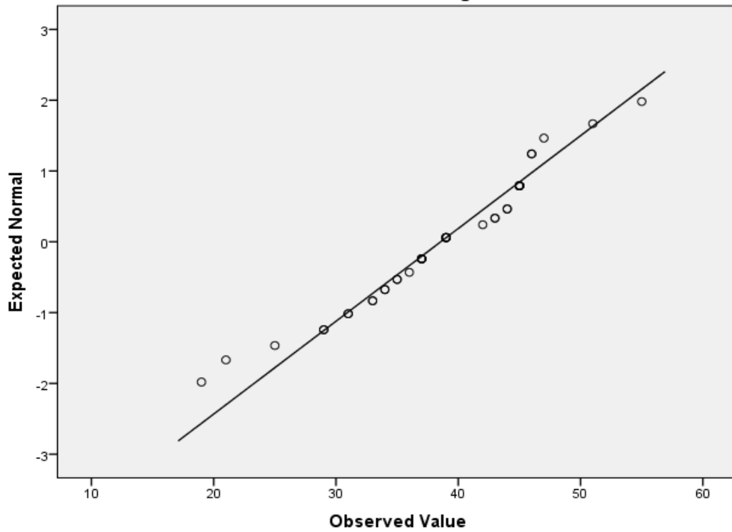
Normal Q-Q Plot of Perkembangan Sosial
