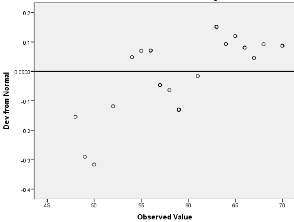
Detrended Normal Q-Q Plot of Peran Orang Tua
