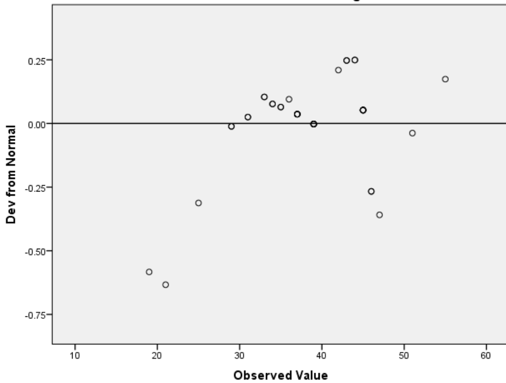
Detrended Normal Q-Q Plot of Perkembangan Sosial
