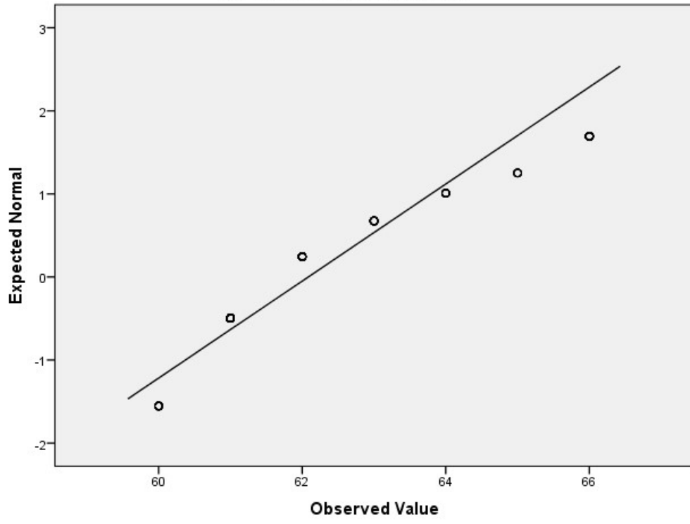
Normal Q-Q Plot of VAR00001
