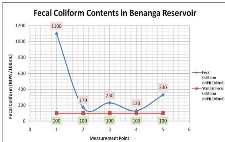
Fig. 5. Water Quality Result of Biological Parameter is Fecal Coliform
