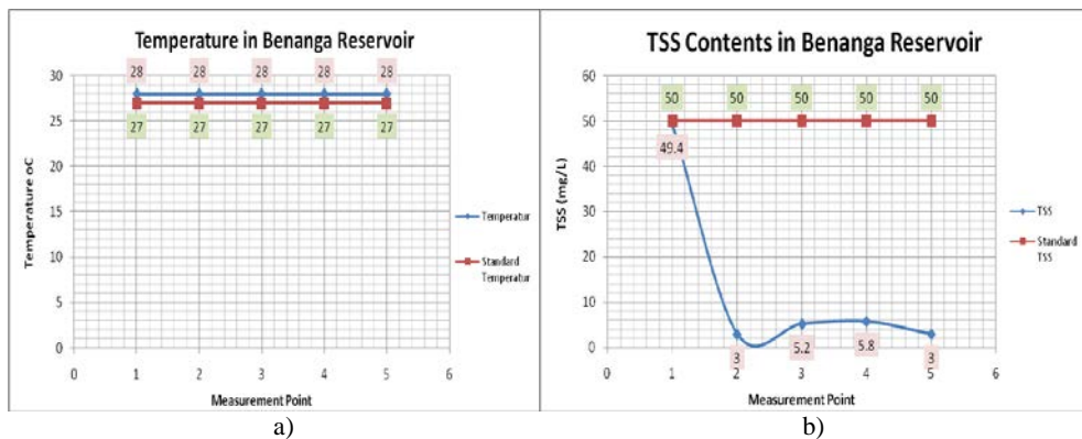
Fig. 3. Water Quality Result of Physical Parameters: a) Temperature and b) TSS
